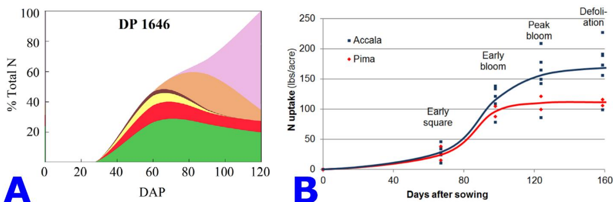
Figure: Seasonal N uptake in cotton reported (A) Texas [5] and (B) California [6].
