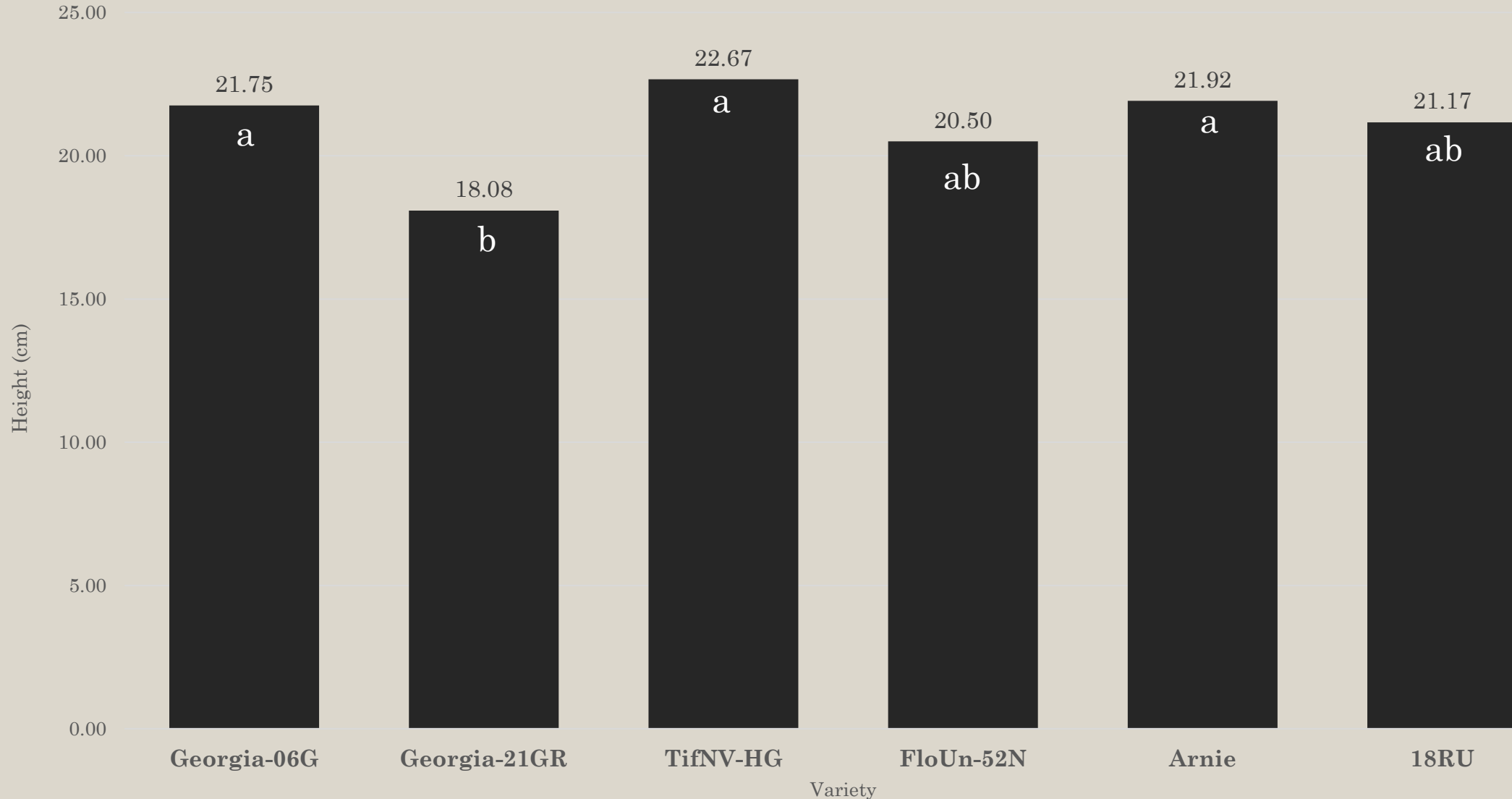
Average Mainstem Height (cm)
