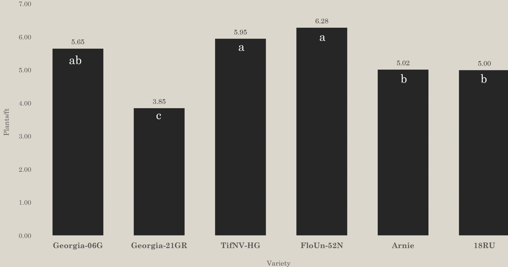
Stand Count Averages
