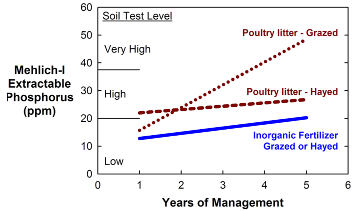
Figure 2. Fertilizer source and management effects on soil test phosphorus in NE Georgia bermudagrass fields.
