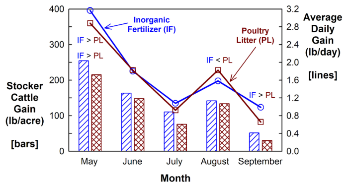
Figure 5. Stacker cattle gain and average daily gain on Coastal bermudagrass fertilized by poultry litter and ammonium-nitrate.
